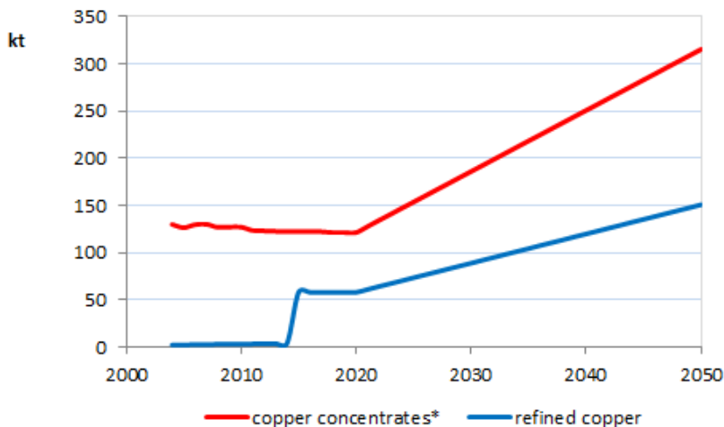
Figure 5-7: Projections of Mongolian copper production in the reference case
